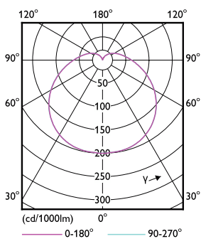
Light Distribution Diagram - TForce Core HB 2Klm 23W E27 865
