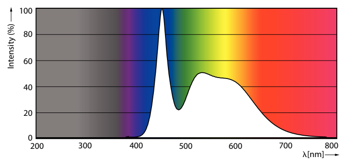
Spectral Power Distribution Colour - TForce Core HB 2Klm 23W E27 865
